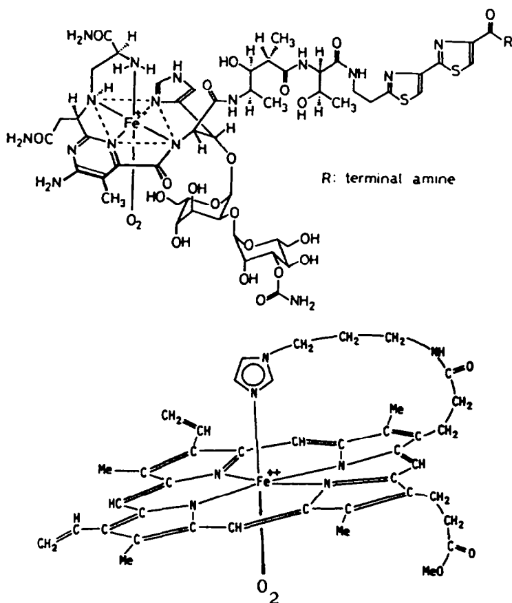
Fig. 1. Iron-bleomycin (upper) and chelated protoheme (lower).
