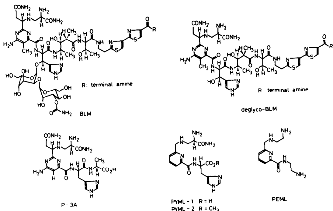
Fig. 3. Biosynthetic intermediates and synthetic analogues of bleomycin.
