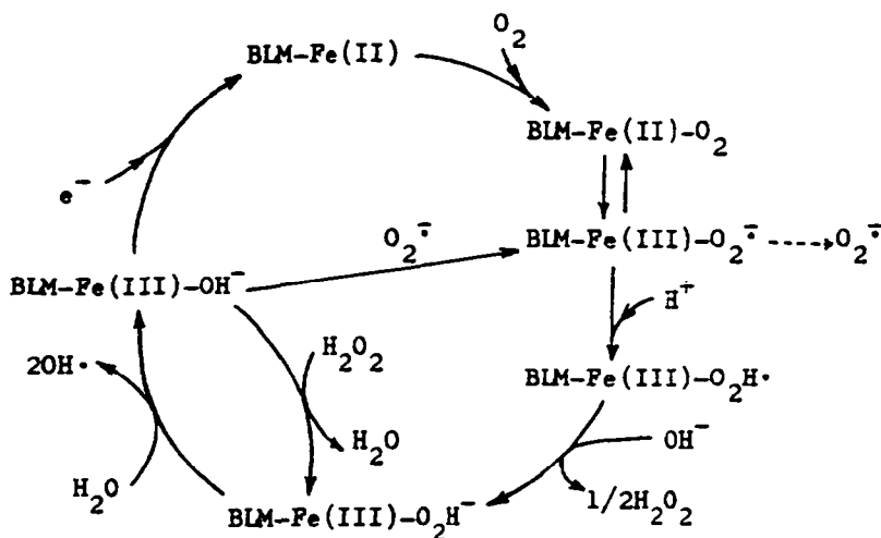
Fig. 2. Hypothetical mechanism for cyclic function of bleomycin-iron complex.
